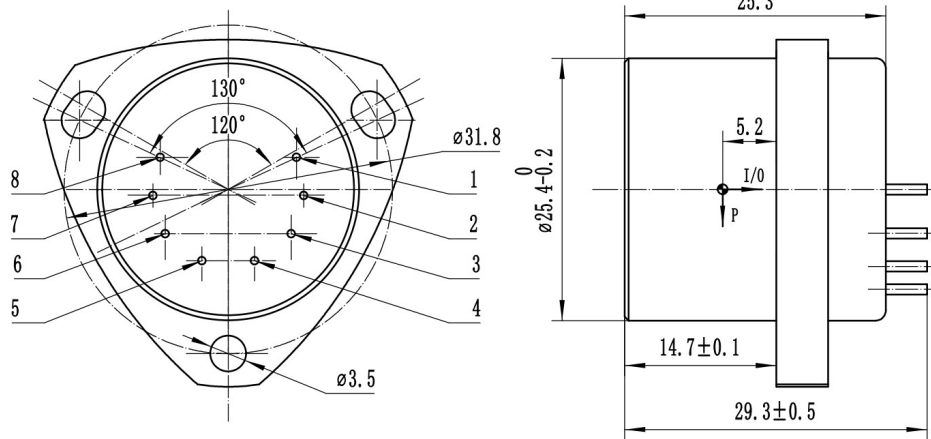
Install hole is U type, pin number is 8
