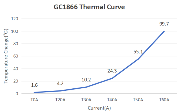
Figure 2. Thermal Curve
