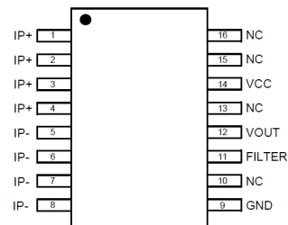
Figure 4. Mode B Pin Diagram
