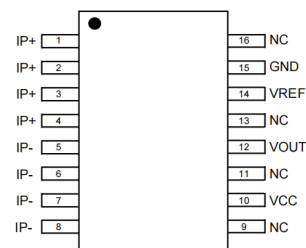
Figure 3. Mode A Pin Diagram
