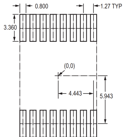
Figure 13. Recommend pad size
