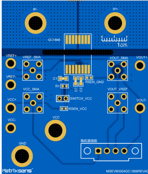
Figure 10. The front of the demo board
