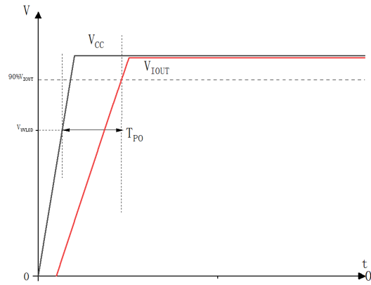
Figure 7. Power-On Time T_{PO}
