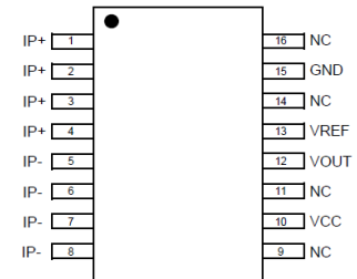
Figure 5. Mode C Pin Diagram
