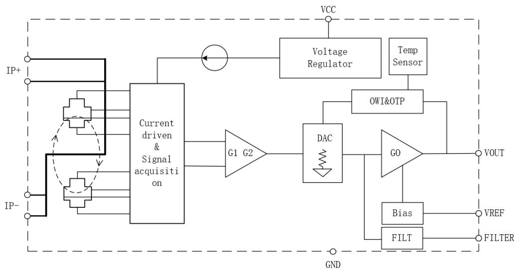
Figure 6. Functional Block Diagram
