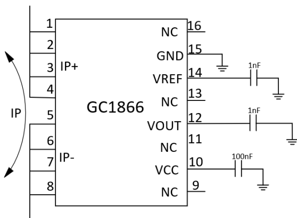
Figure 1. Typical Application Circuit Diagram Of Type A
