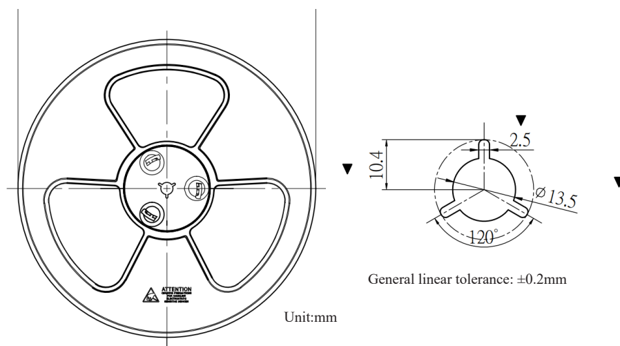
Figure 14. Tape rules
