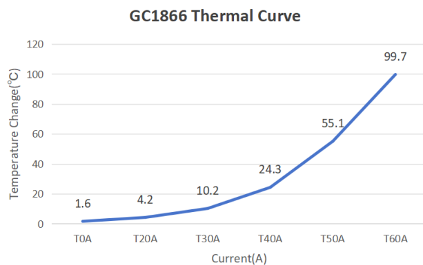
Figure 9. Thermal curve
