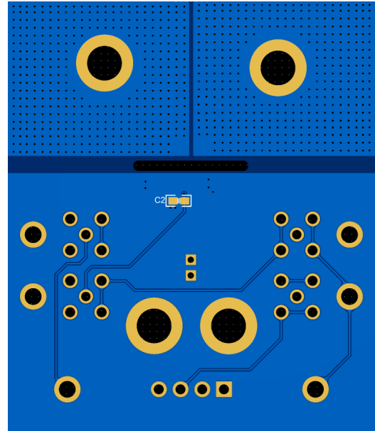
Figure 11. The back of the demo board
