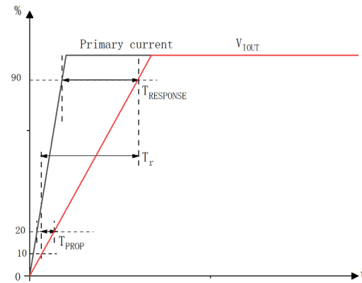
Figure 8 . Dynamic Response Time Parameters
