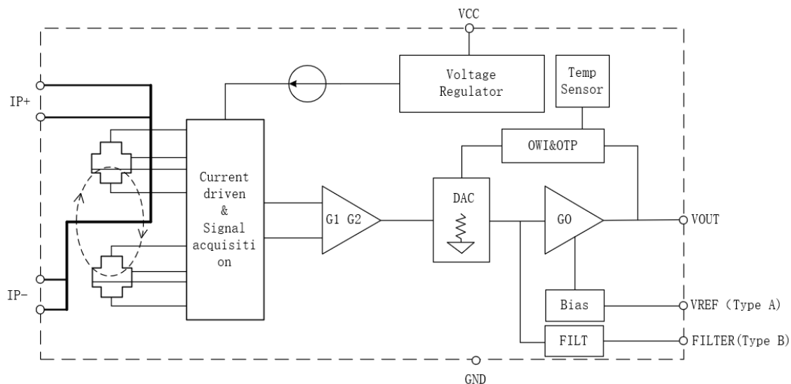
Figure 5. Functional Block Diagram
