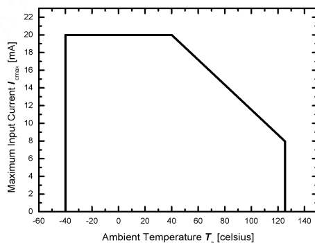
Figure 1. Maximum input current I_{cmax}
