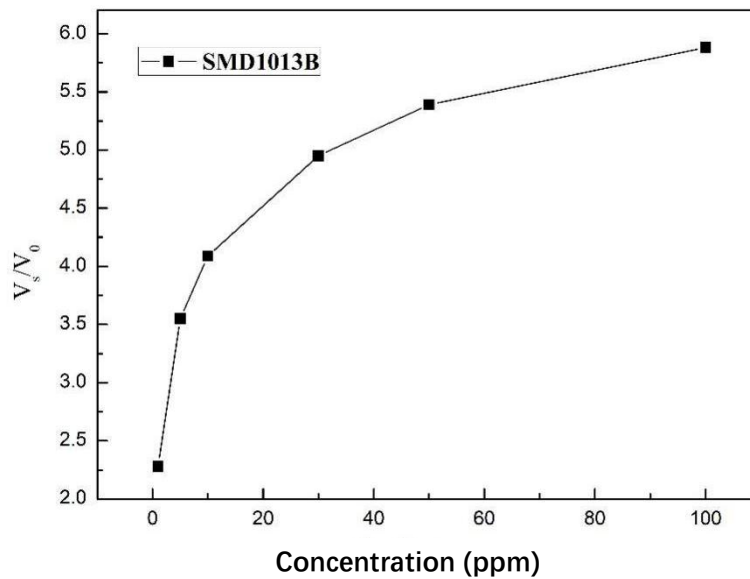
Figure 1 Sensor sensitivity characteristic curve
